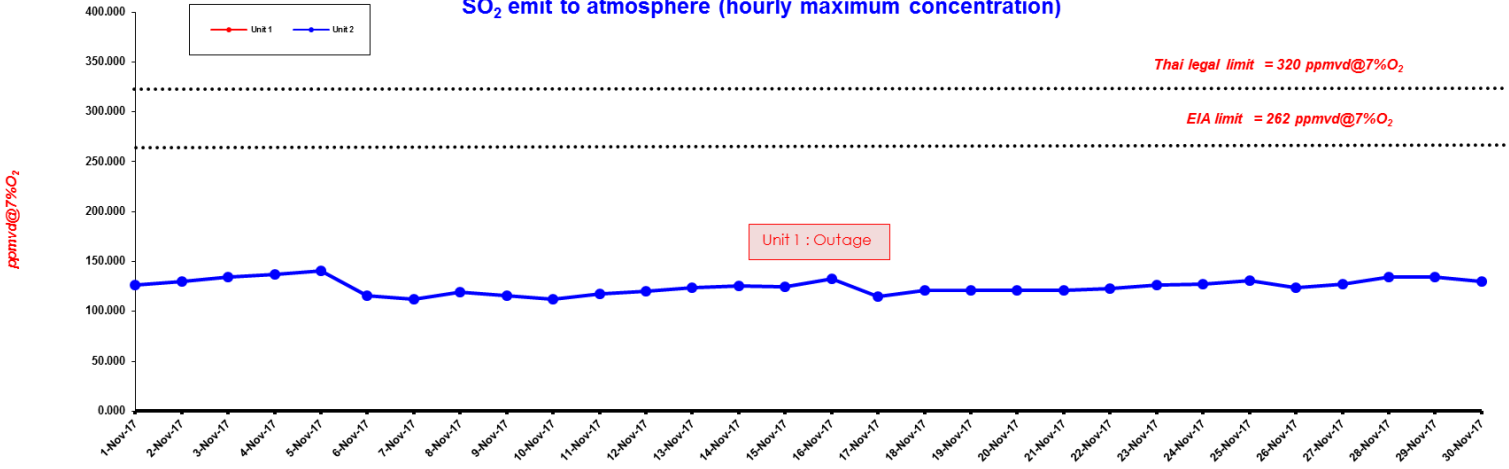
SO 2 emit to atmosphere (hourly maximum concentration)
